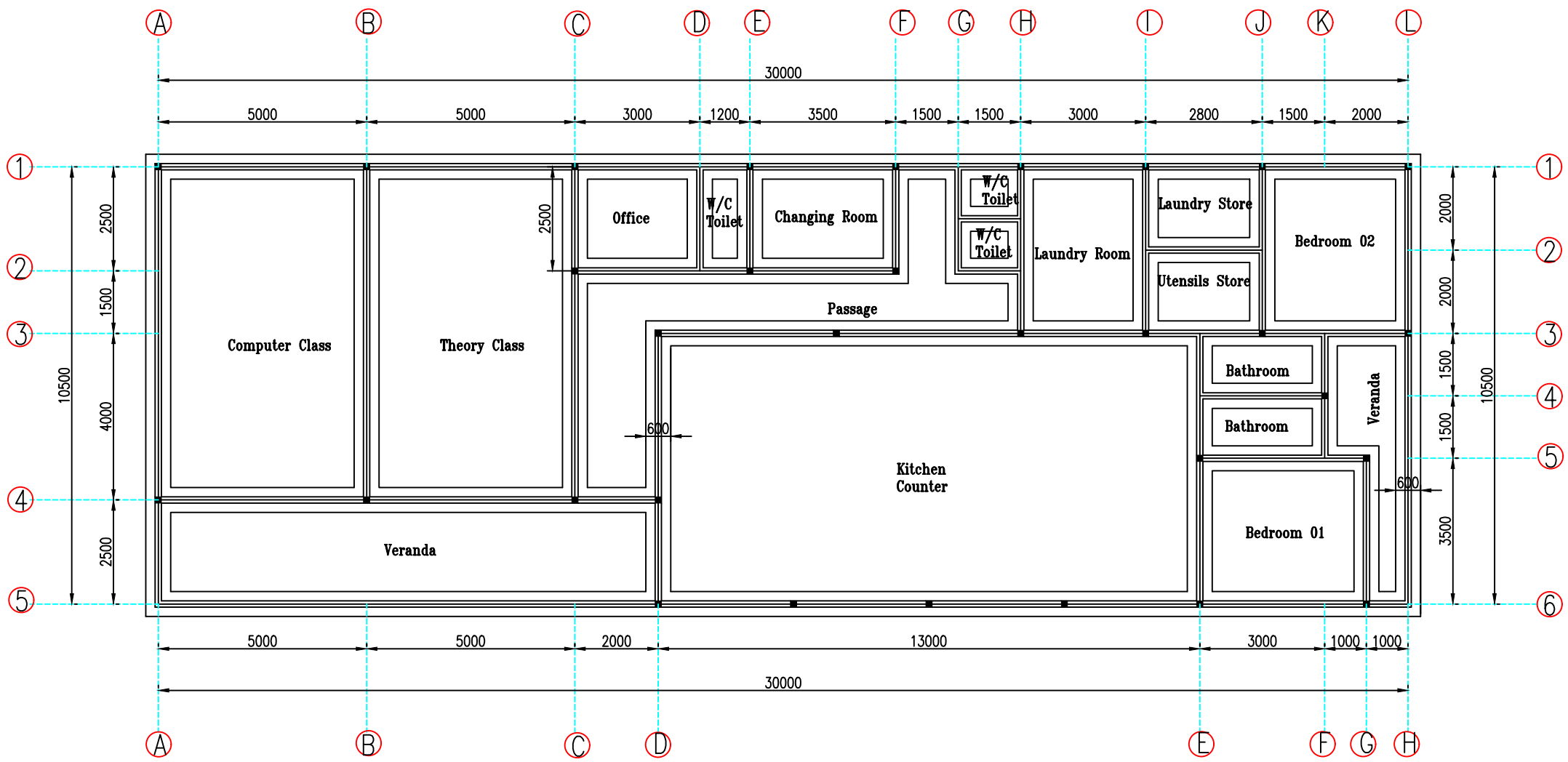
FOUNDATION PLAN
